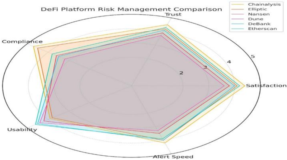
Figure 3. DeFi_Platform_Radar_Chart
